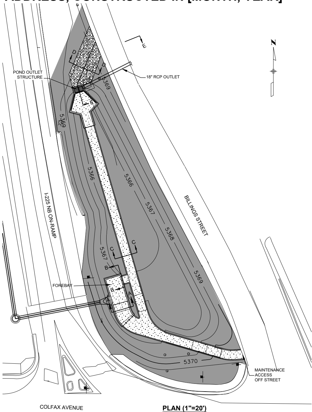
PLAN (1"=20')
