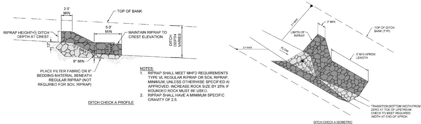
Figure 5.05.1. Ditch Check Schematic
