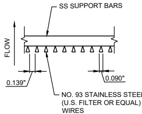
WATER QUALITY TRASH RACK NTS
