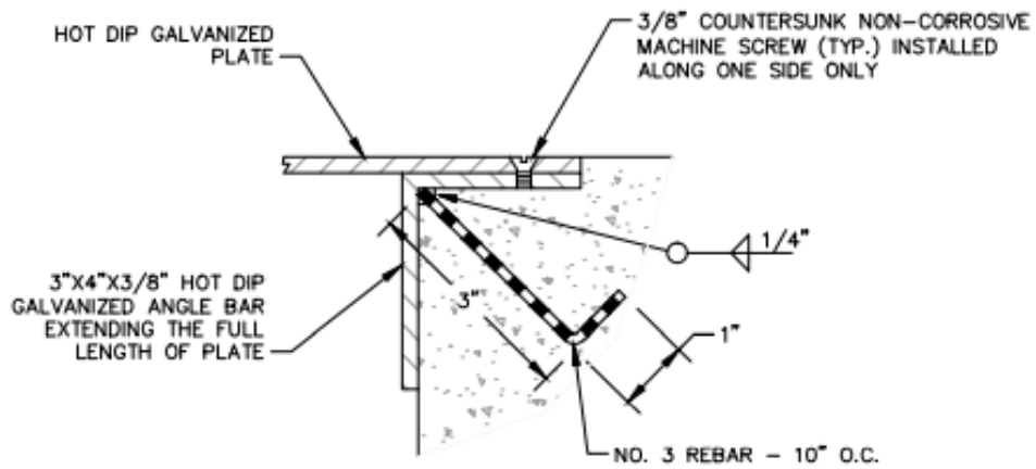
DETAIL "A"
